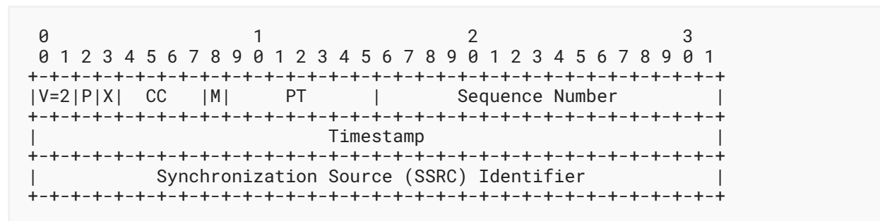
Figure 6: RTP Header
